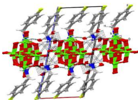
Figure 1 : Selected relevant hydrogen bonds structure within the crystal packing
