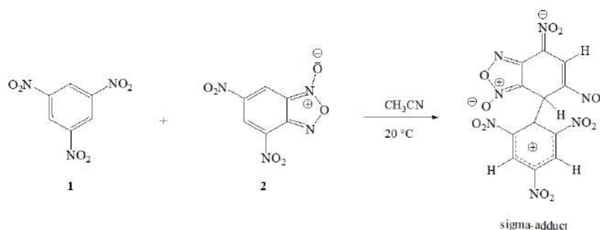
Reaction of 1, 3, 5-trinitrobenzene 1 with the superelectrophile 4,6-dinitrobenzofuroxan 2
