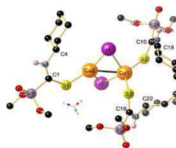
Figure. Molecular structure of C1 .
