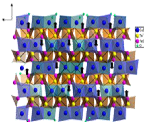
Projection on the bc plane of the chaine of polyhedra
