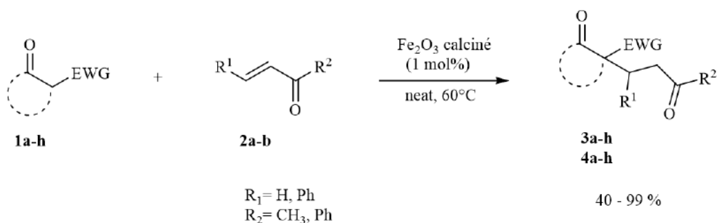
Scheme 1. Michael addition of 1,3-dicarbonyl onto \alpha,\beta -unsaturated carbonyl compounds
