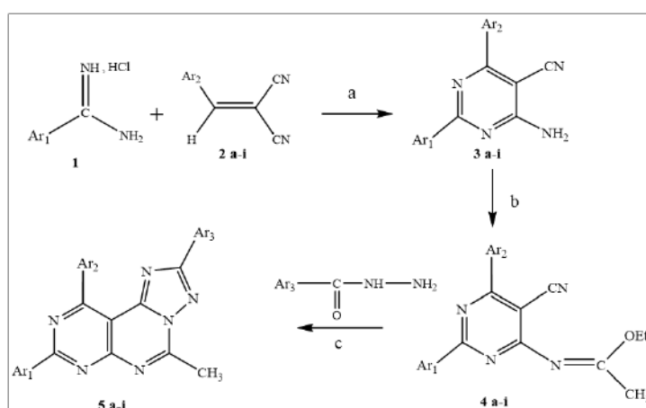
Scheme 1: Synthesis of triazolopyrimidopyrimidines 5a-i , Reagents and conditions:
