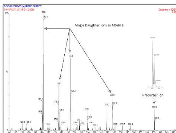
Fig. 1: MS/MS spectra of Chloramphenicol in Daughter Scan mode
