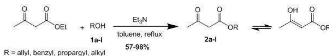
Scheme 1. \text{Et}_3\text{N} -mediated transesterification of ethyl acetoacetate with various alcohols
