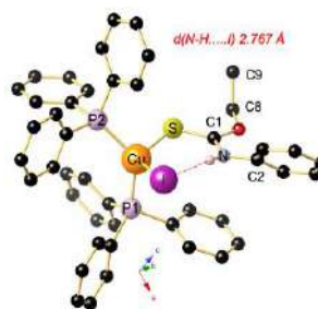
Figure. Molecular structure of C8 .
