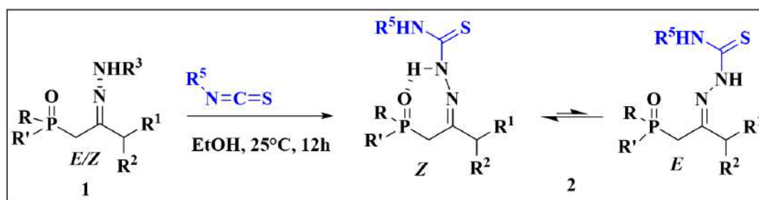
Fig I: Synthesis of phosphonated thiosemicarbazone ligands
