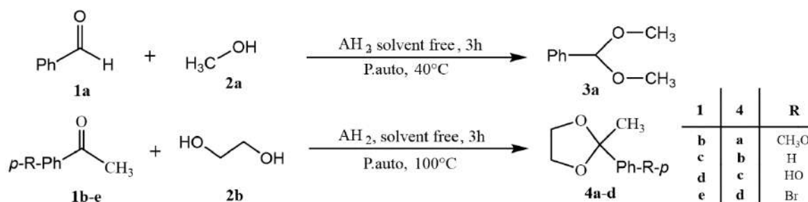
Scheme: Synthesis of cetal 3a and 1,3-dioxolanes 4a-d from carbonyl compounds 1a-e .
