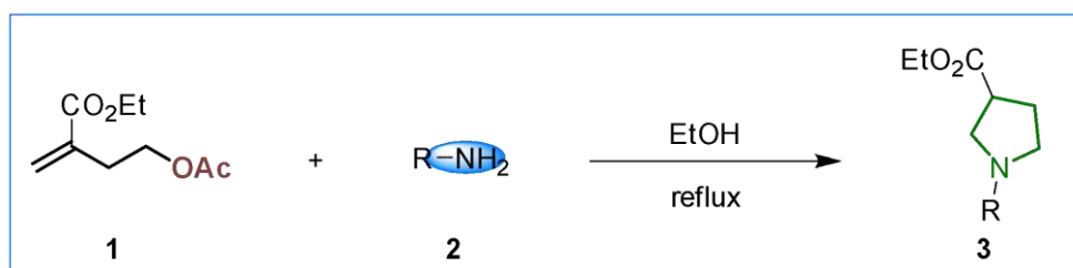
Scheme: Aza-Michael addition of primary amines to homoallylic living group (acetylated).
