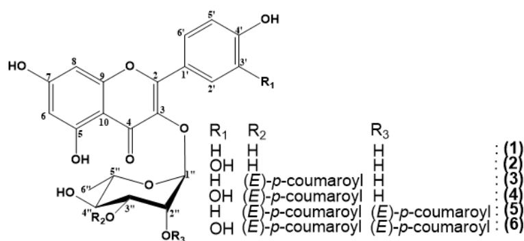
Figure 1. Structures of the isolated flavonoid glycosides from F. tunetana .
