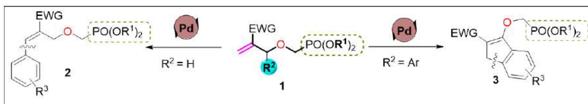
Scheme: Heck coupling reaction on dialkyl allyloxymethylphosphonate
