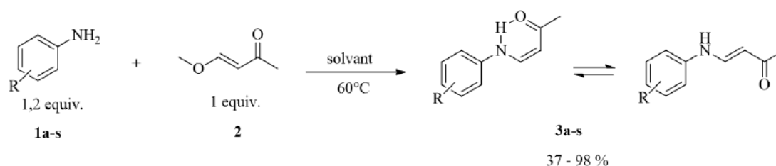
Scheme 1 : Aza-Michael additions of anilines onto 4-methoxy-3-buten-2-one
